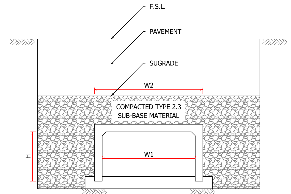
BOX CULVERT INSTALLATION DETAIL*
