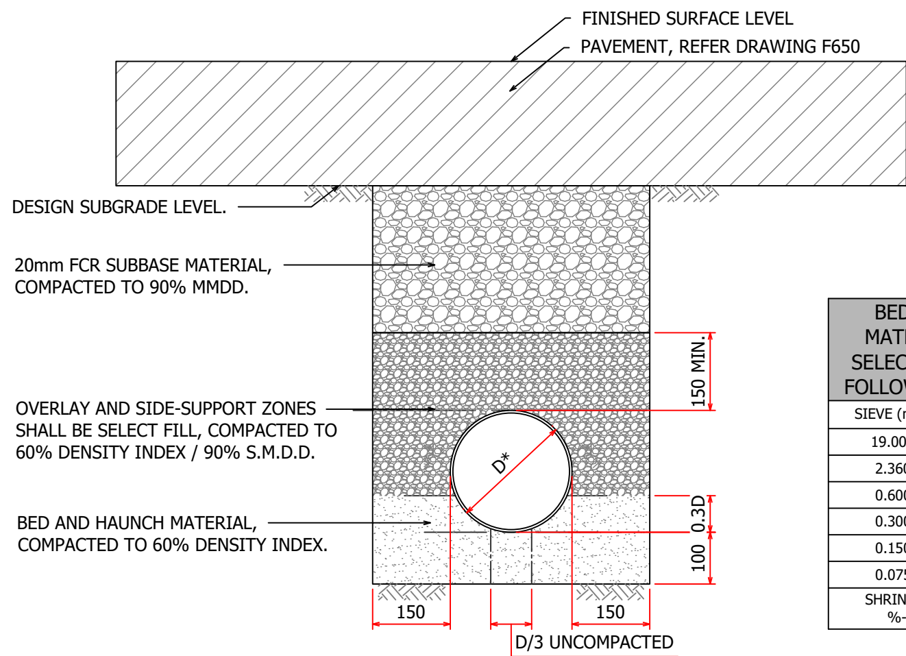
RCP PIPE INSTALLATION TYPICAL DETAIL N.T.S.
