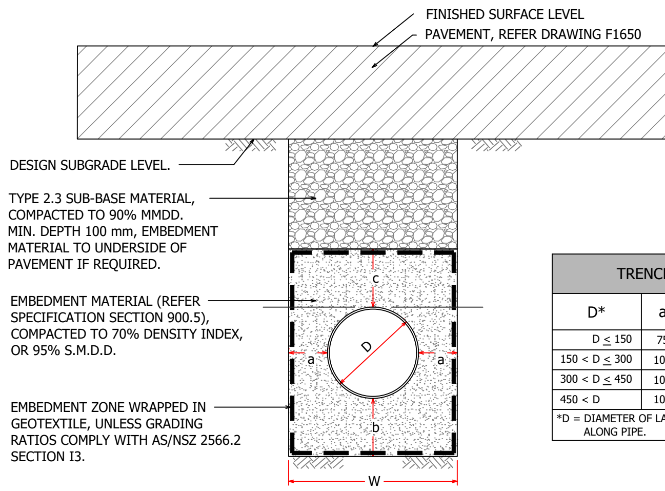
PVC-U AND PP PIPE INSTALLATION TYPICAL DETAIL N.T.S.
