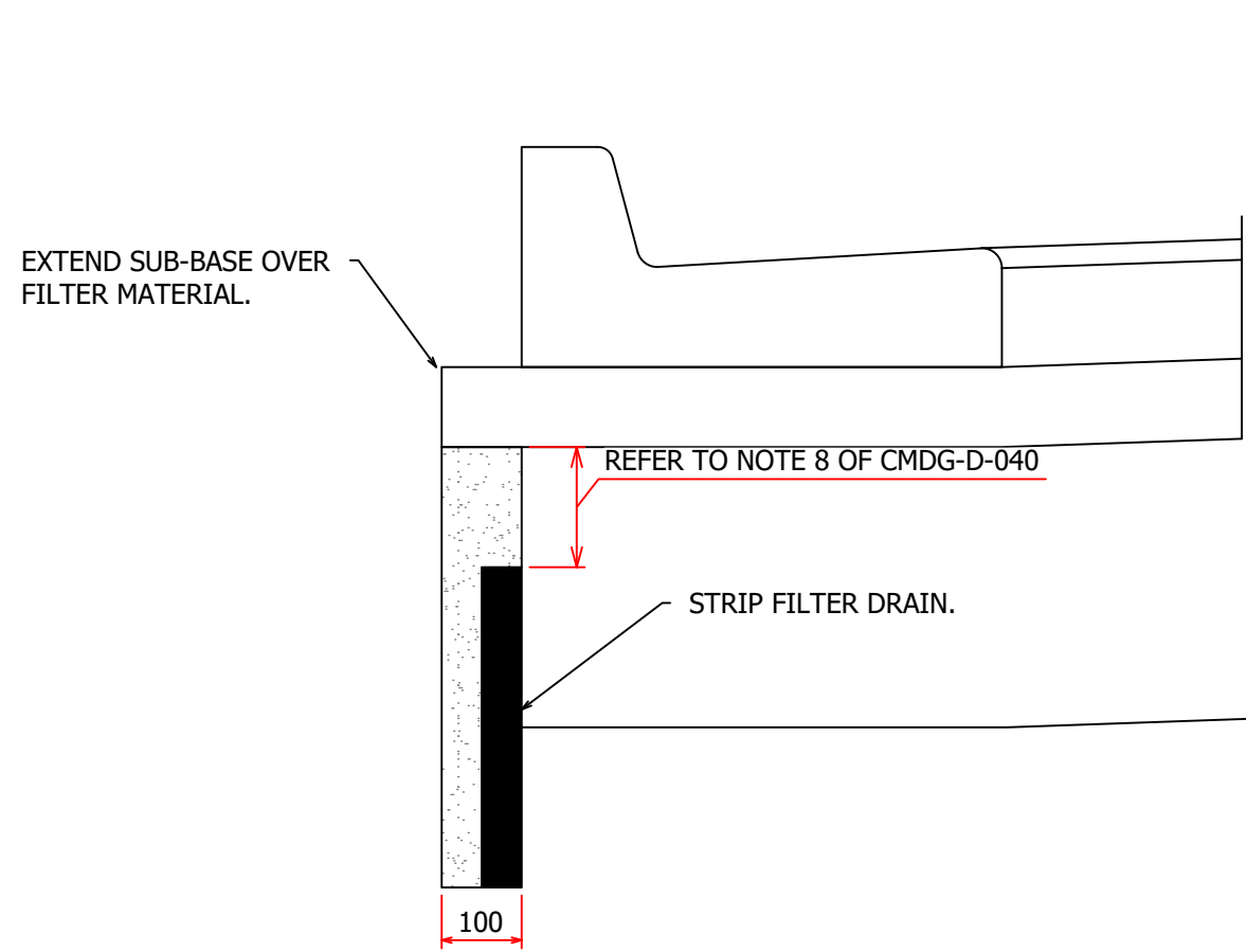
TYPE 2 SUBSOIL DRAINAGE BEHIND KERB TYPICAL DETAIL*
